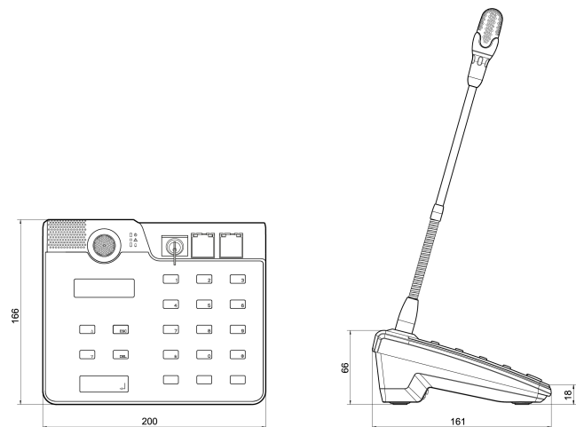
Dimensions of Call Station
