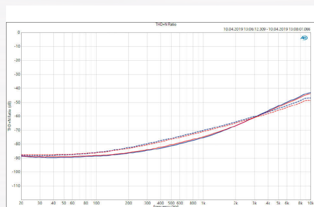
ABB. 11: Distortion factor (THD+N) with 8 \Omega (solid line) and 4 \Omega (--) load depending on frequency at 300 W per channel (x-axis).
