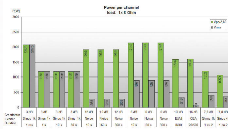
ABB. 15: Performance values at 8 \Omega with simultaneous loading of all channels (upper graphic) and loading of only one channel (lower graphic)
