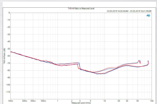
ABB. 09: Distortion factor (THD+N) at 1 kHz with 8 \Omega (solid line) and 4 \Omega (--) load depending on the output voltage [x-axis]. The small jump at 3 V occurs when switching from normal operating mode back to eco mode.
