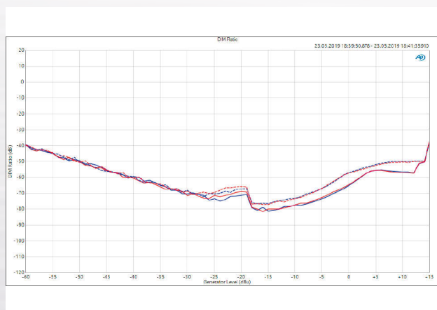
ABB. 12: DIM measurement with 8 \Omega (solid line) and 4 \Omega (--) load (CH2, CH6) depending on the input level (x-axis).
