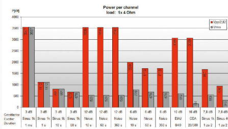
ABB. 14: Performance values at 4 \Omega with simultaneous loading of all channels (upper graphic) and loading of only one channel (lower graphic)
