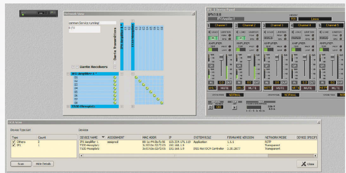
FIG. 01: The IRIS-Net surface with Dante configurator (top left), OCA scan (bottom) and the IPX amplifier's user interface (top right).
