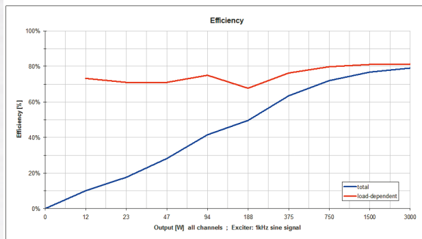
ABB. 16: Amp efficiency in % as a function of the power output [x-axis]. In red, the curve without base load showing the amplifier's very good efficiency.
