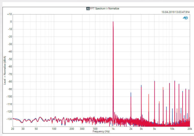
ABB. 10: Output signal as a spectrum at 1 kHz with 8 \Omega load and 600 W per channel.
