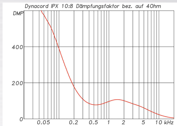
ABB. 07: Damping factor related to a 4-Ω load. Illustrated for channel 1. At 1 kHz, the damping factor is 100. In the important low-frequency range below 200 Hz, values of 200 and more are reached.
