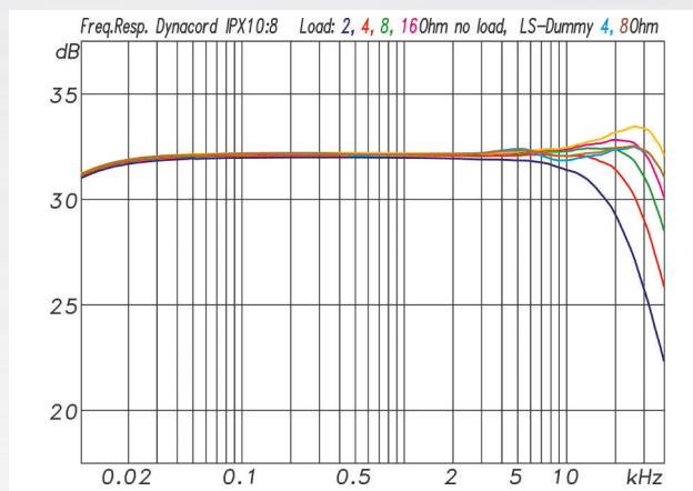
FIG. 06: Frequency response with 2, 4, 8 and 16 Ω loads, without load and with 4 or 8 Ω loudspeaker dummy loads.
