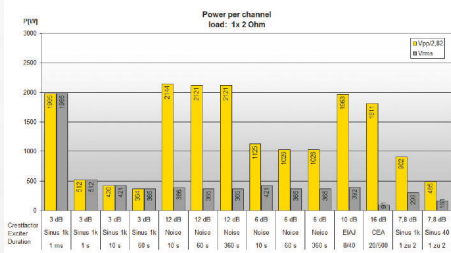
ABB. 13: Performance values at 2 \Omega with simultaneous loading of all channels (upper graphic) and loading of only one channel (lower graphic)
