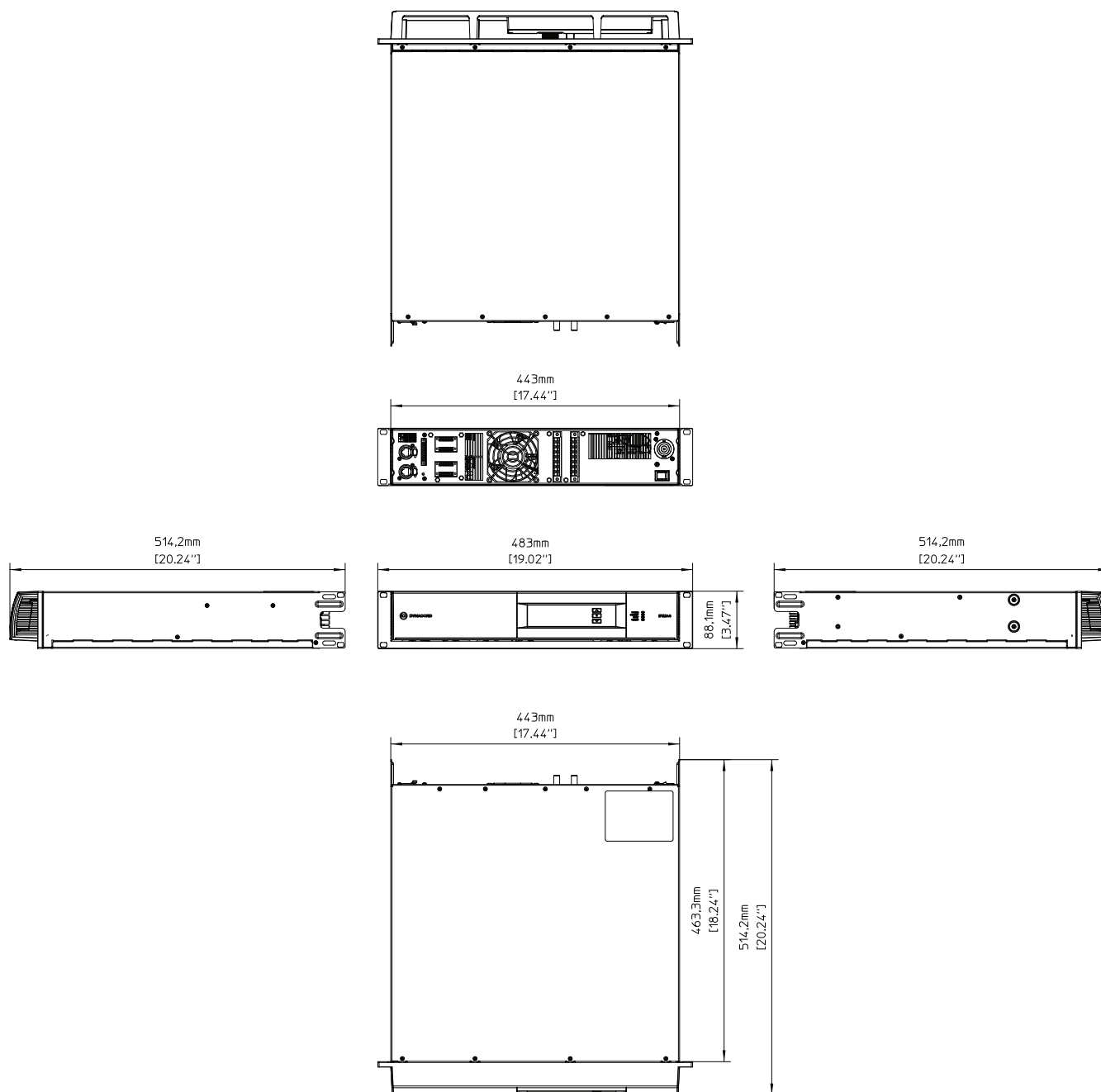
Figure 8.2: Dimensions: IPX
