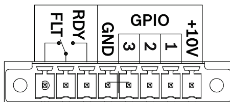
Figure 6.3: Control port
