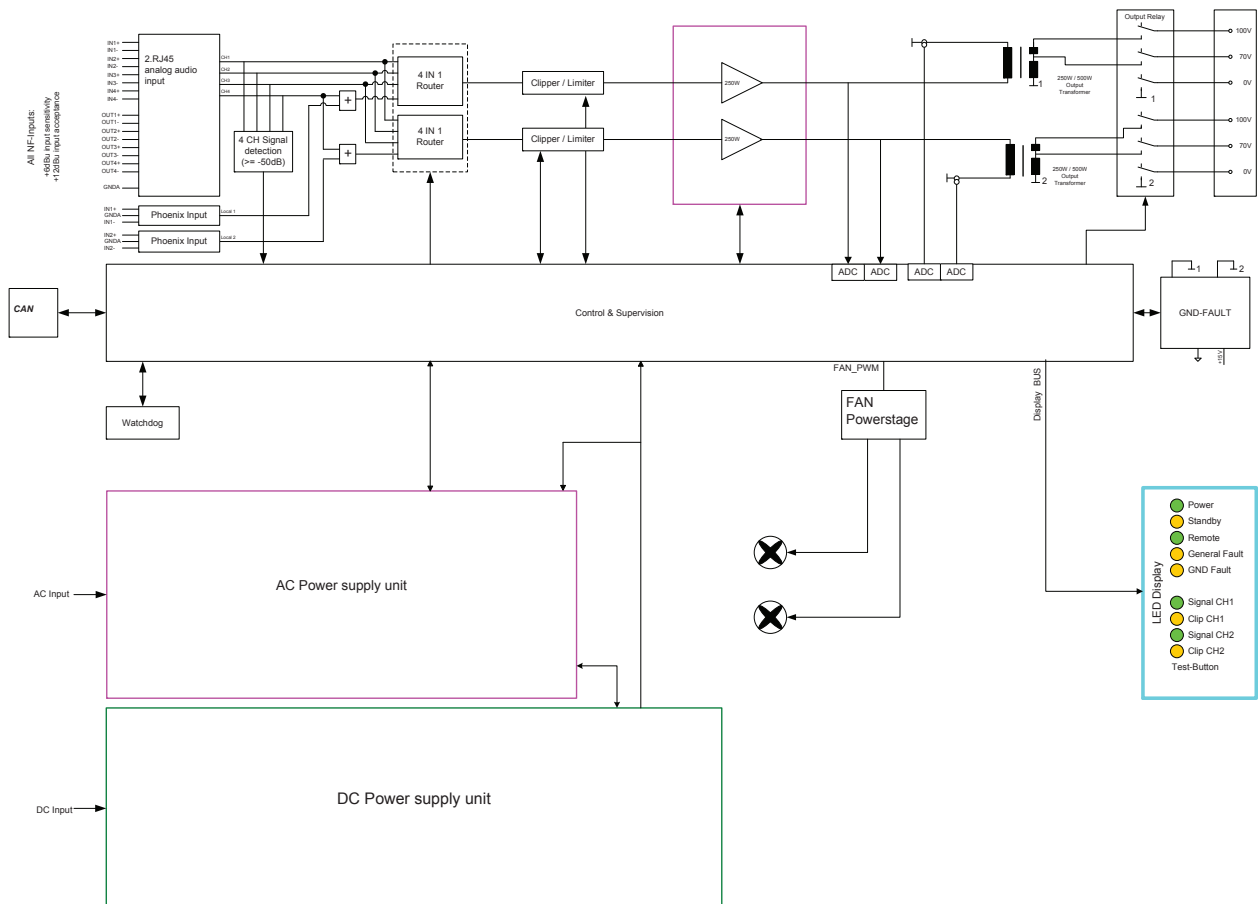
Circuit diagram
