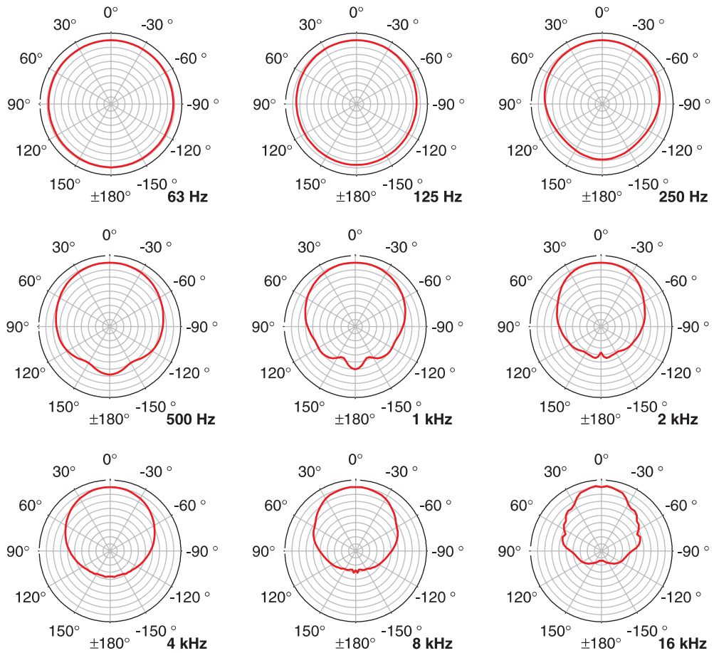
Horizontal Directivity, 5dB/Div, 50dB Radius, 1/1 Oct.
