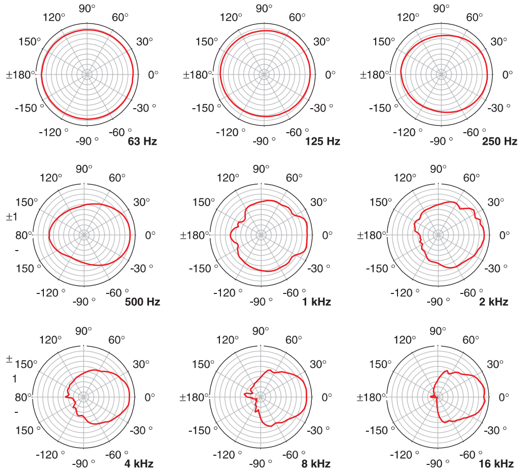
Vertical Directivity, 5dB/Div, 50dB Radius, 1/1 Oct.
