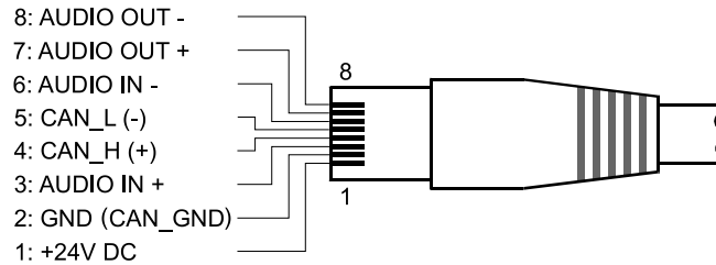
Figure 6.3: Assignment of the PCA bus connector
