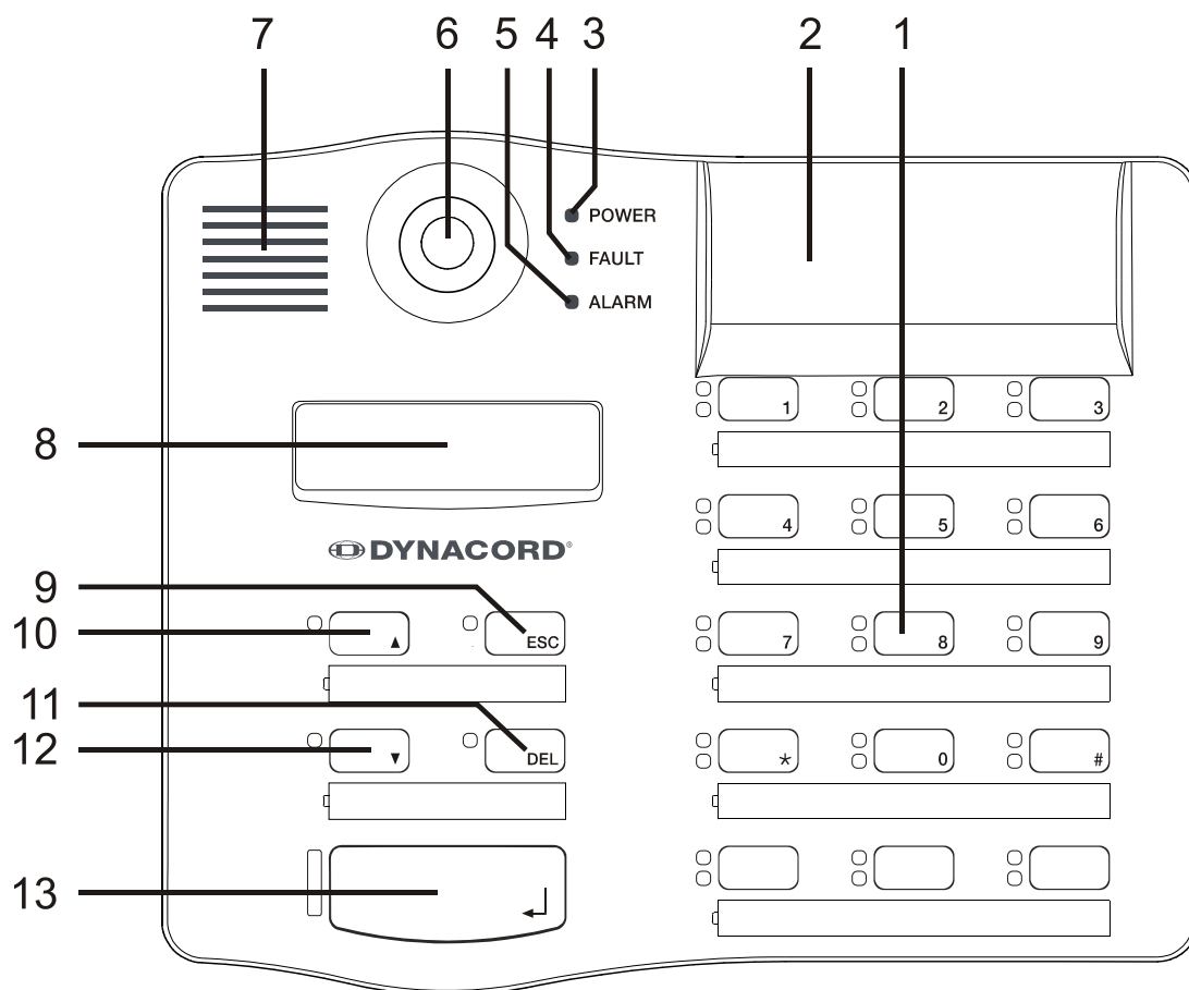
Figure 5.1: DPC 8015
