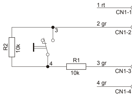
Figure 5.7: Connecting NRS 90231
