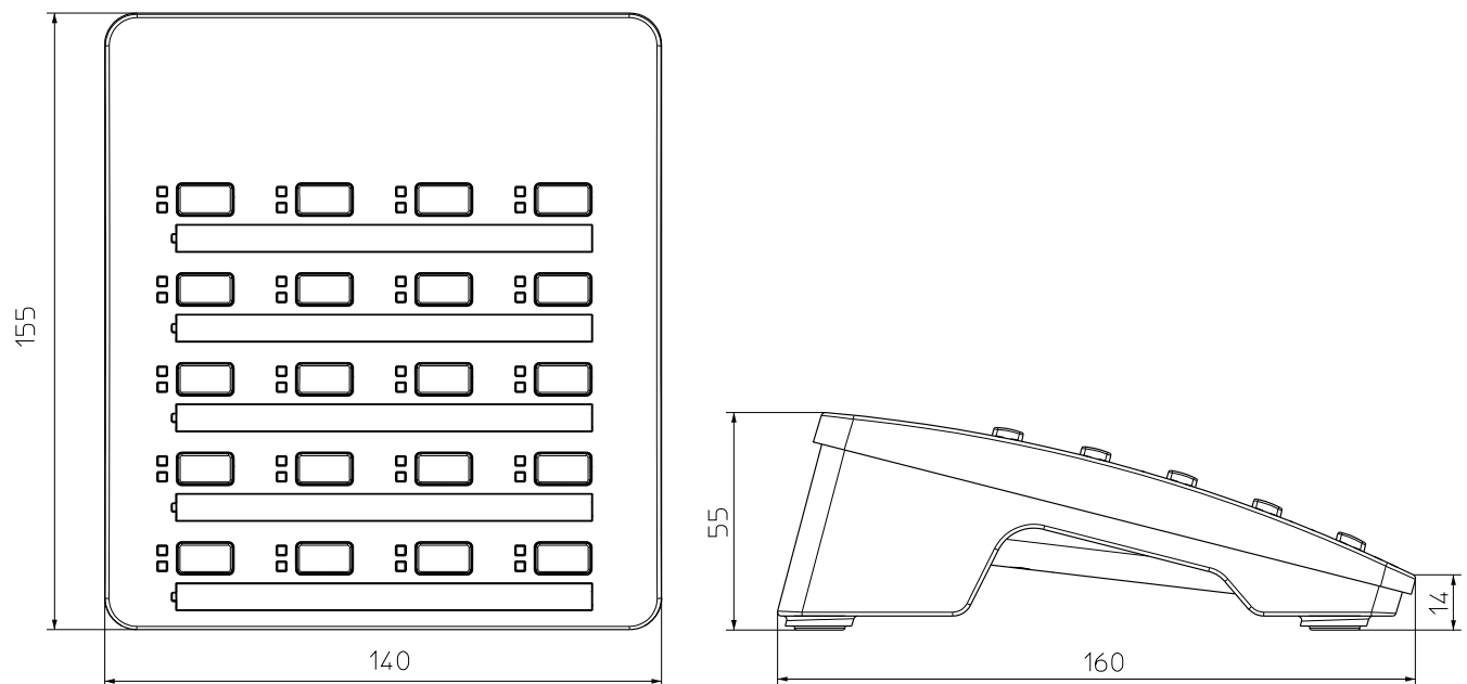
Figure 10.2: DPC 8120
