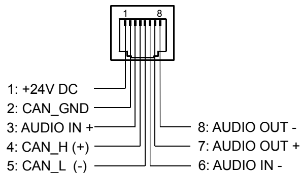
Figure 6.2: Assignment of the PCA bus interface
