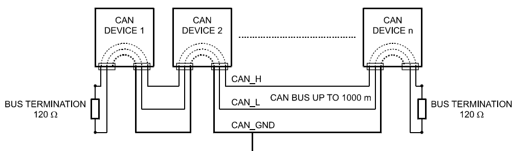
Figure 11.1: CAN bus
