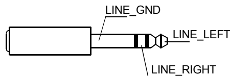
Figure 6.4: Assigning the LINE plug as audio input
