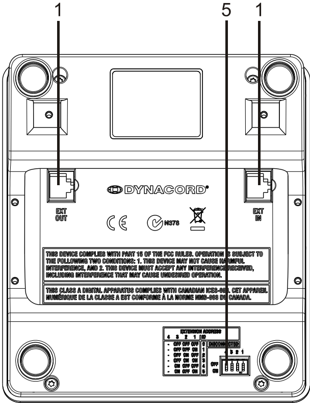
Figure 5.4: DPC 8120
