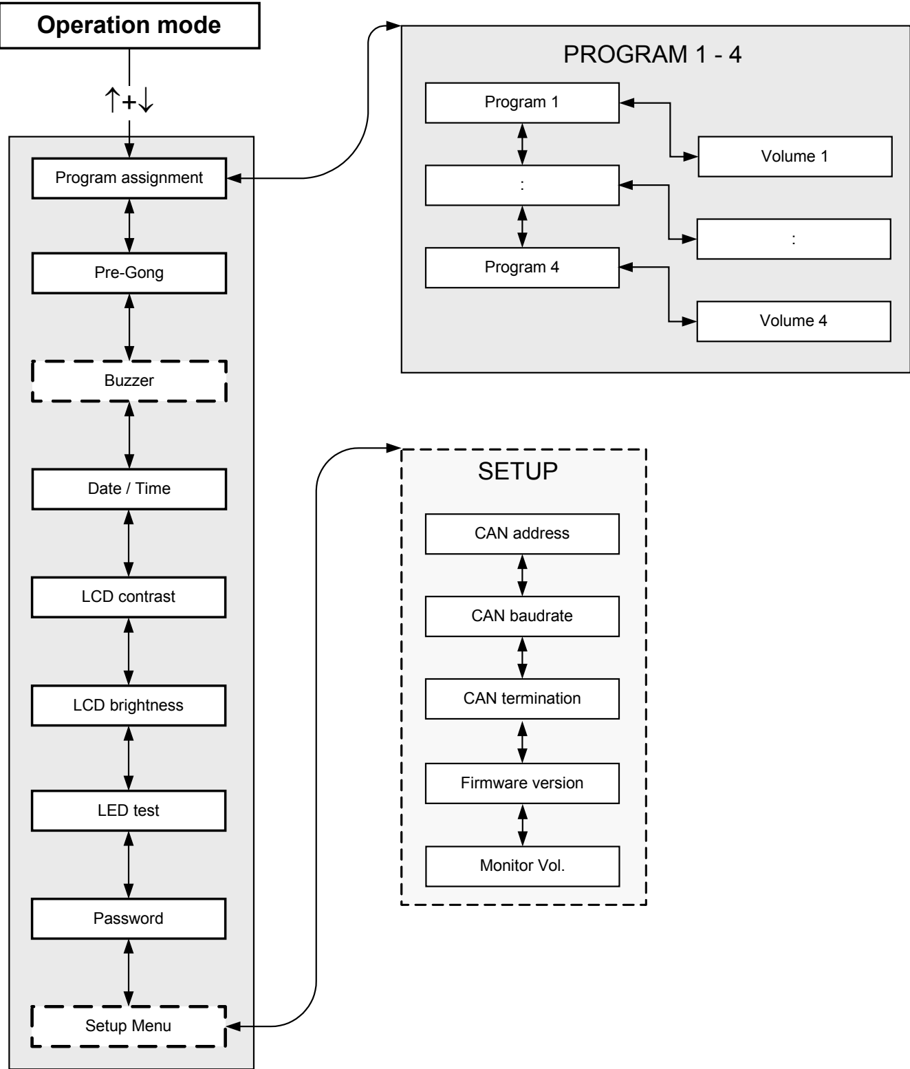
Figure 7.1: Menu structure
