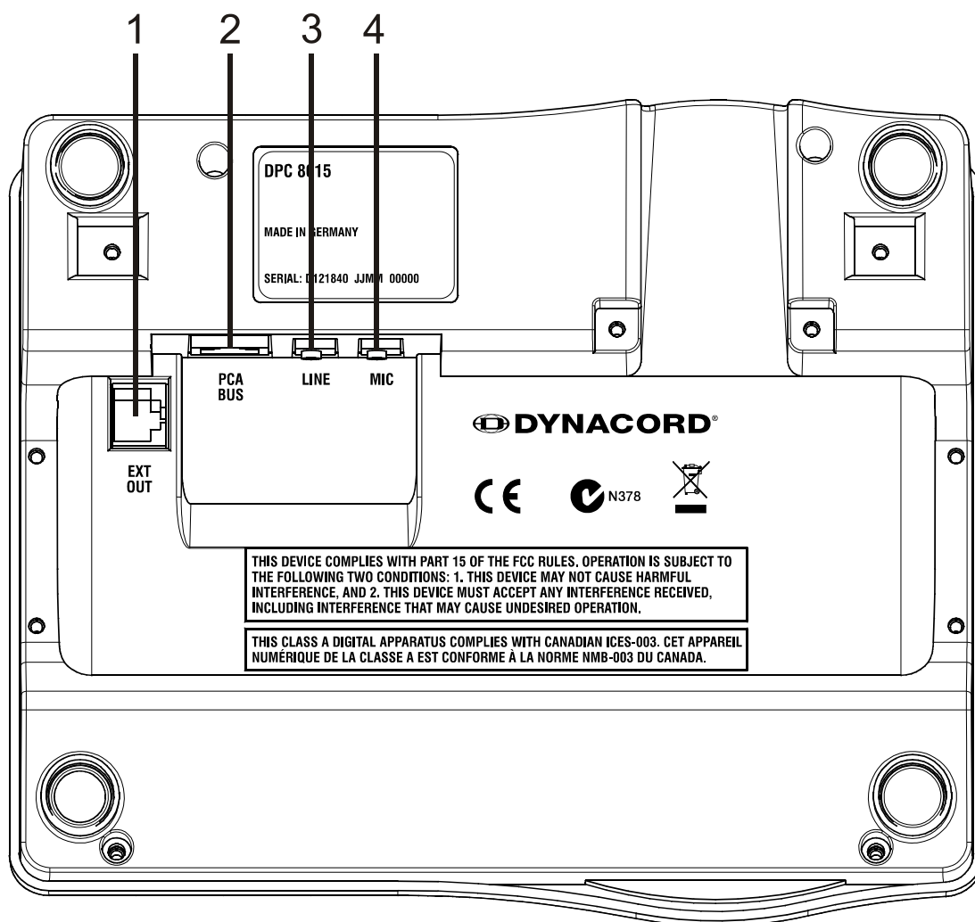
Figure 5.3: DPC 8015
