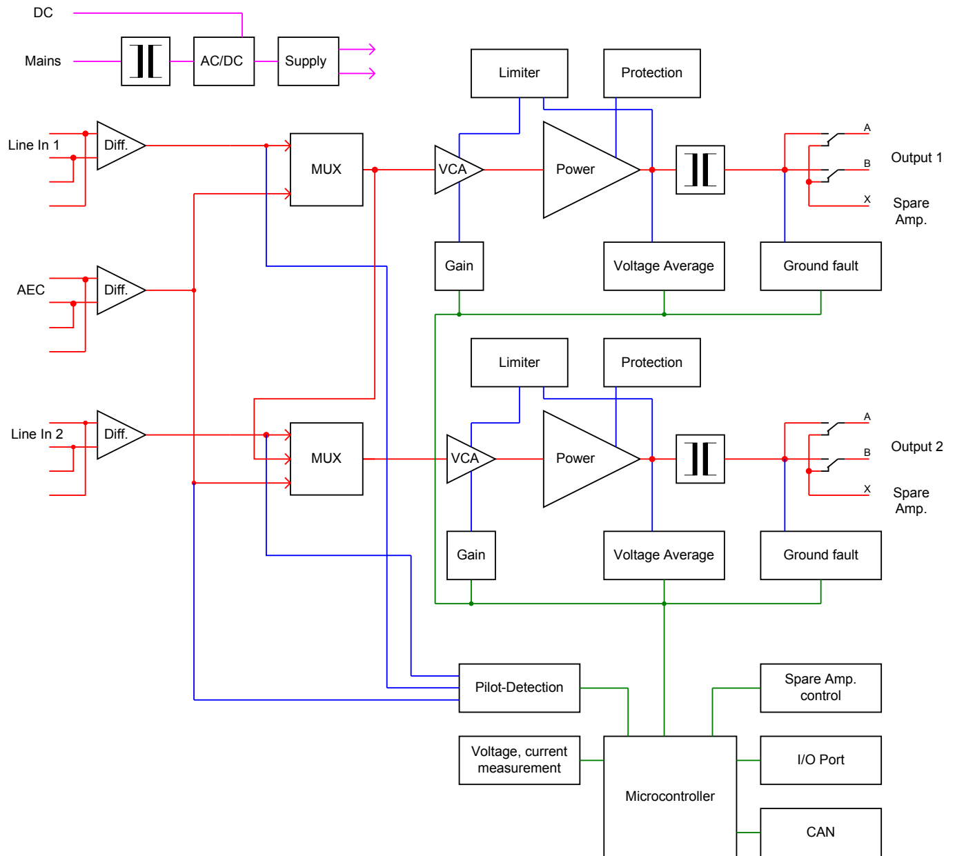
Block diagram (diagram shows DPA 8225)
